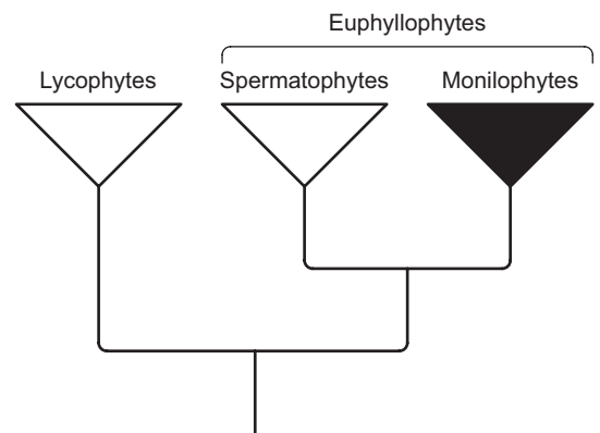
Fig. 1. Consensus phylogeny depicting relationships of major vascular plant lineages. Topology summarizes the results of previously published phylogenetic studies (e.g., Raubeson & Jansen, 1992; Kenrick & Crane, 1997; Renzaglia & al., 2000; Pryer & al., 2001a, see main text for others). Resolved nodes have received bootstrap support \geq 70 .
